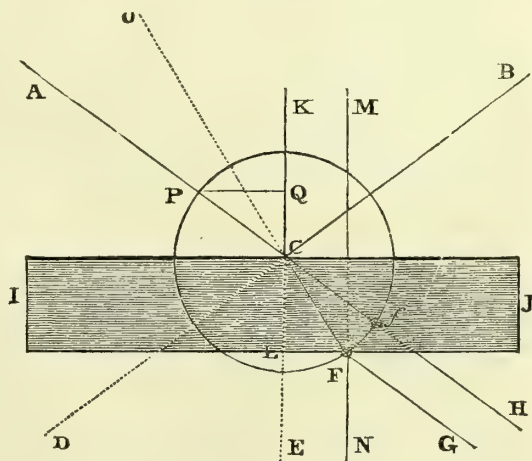
Reflection and Refraction of Light.
